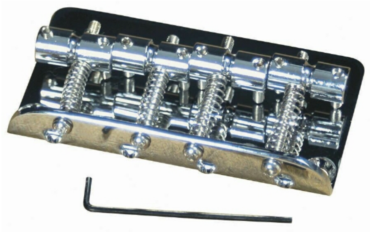
Retro Parts RP255C Bass Bridge
