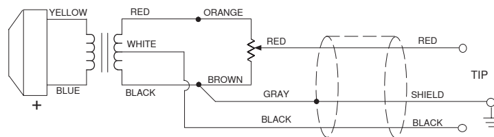
INTERNAL CONNECTIONS UNBALANCED HIGH-IMPEDANCE OUTPUT
